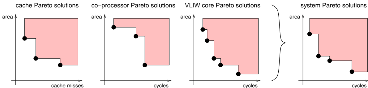
Figure 7: Subdividing the design space into independent parts for optimization.
