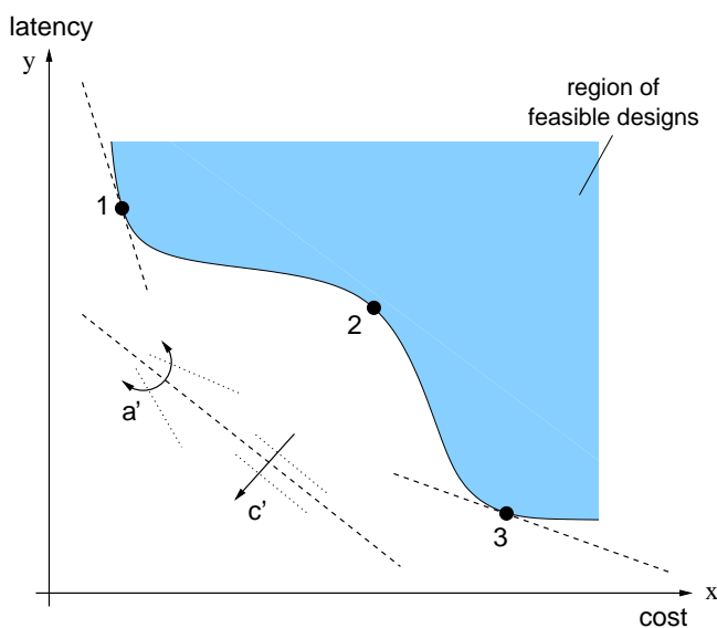
Figure 4: Finding Pareto-optimal designs using a weighted sum of objectives.
